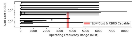
Fig. 1: Operating frequency range for low-cost SDRs.
