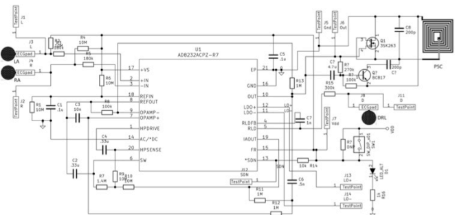
Fig. 2. Schematic diagram of the proposed ECG sensor.
