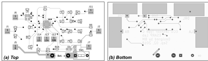
Fig. 3. Layout of the PCB: (a) Top layer and (b) Bottom layer.
