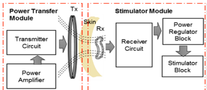
Fig. 2. Block diagram of the stimulator.
