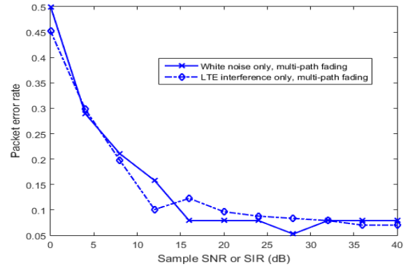
Fig 3. Packet error rate vs. SNR of the 802.11a system, affected by white noise and LTE interferences, respectively.
