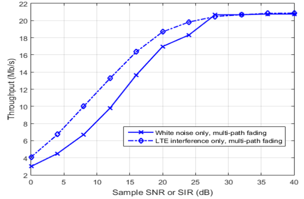
Fig 2. Throughput vs. SNR (or SIR) of the 802.11a system, affected by white noise and LTE interferences, respectively.
